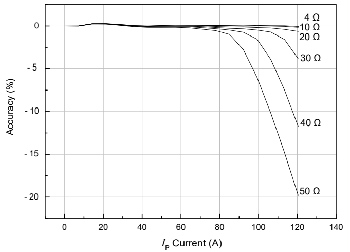
Figure 4: Accuracy @ 60 Hz
