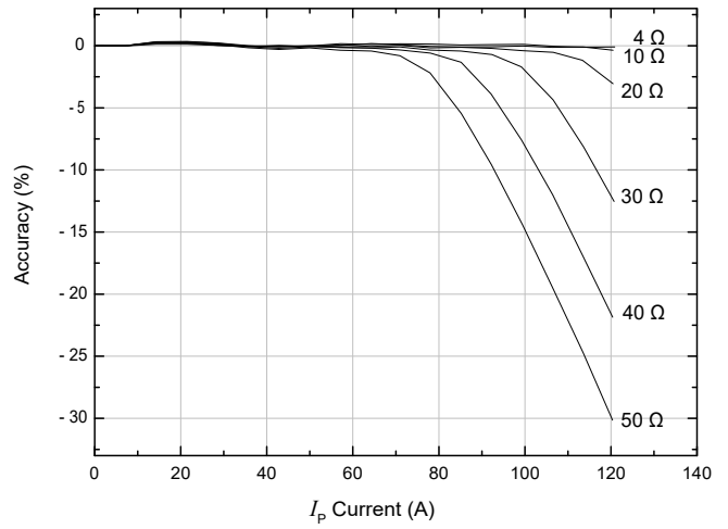
Figure 2: Accuracy @ 50 Hz
