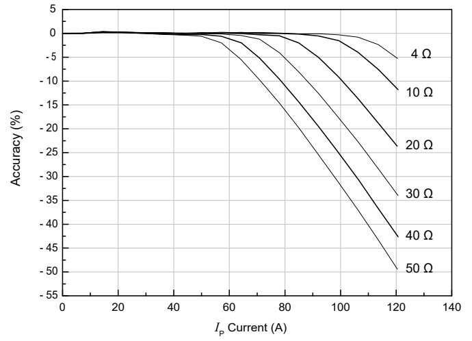
Figure 8: Accuracy with different R_L @ 70 °C
