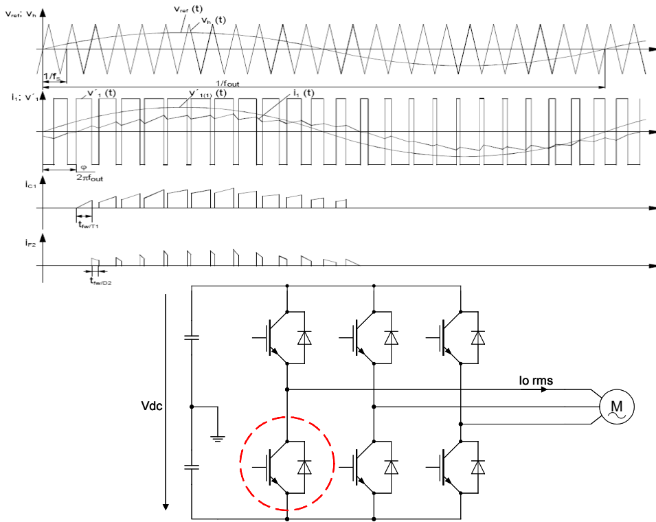
Fig. 30: Definitions, topology and modulation used in the ABB simulation tool.
