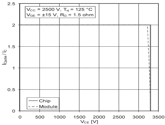
Fig. 18: Turn-off safe operating area (RBSOA)
