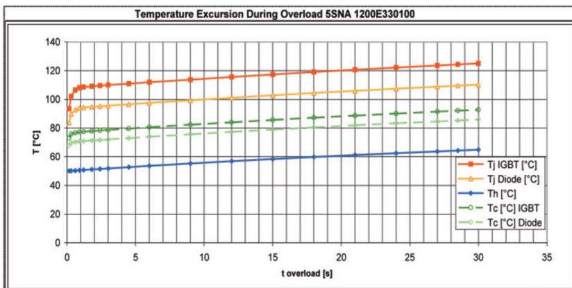
Fig. 36: Output curves showing temperature excursion during the defined overload
