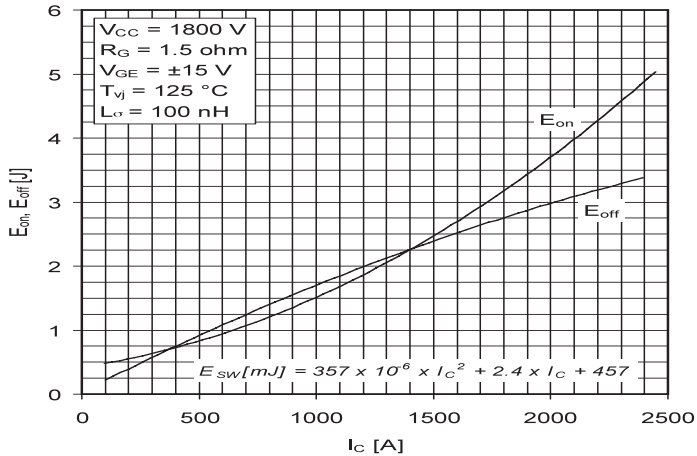
Fig. 12: Typical switching energies per pulse vs. collector current
