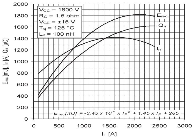
Fig. 19: Typical reverse recovery characteristics vs forward current
