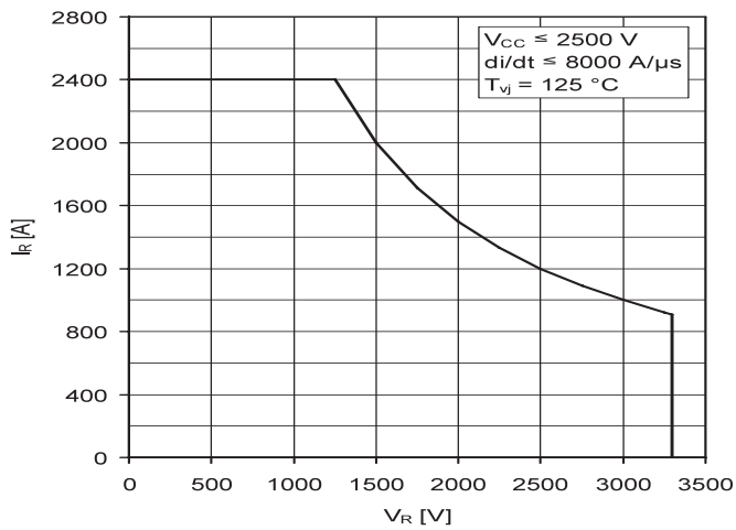
Fig. 22: Safe operating area diode (SOA)
