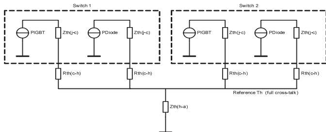
Fig. 27: Thermal equivalent block diagram for devices with baseplate
