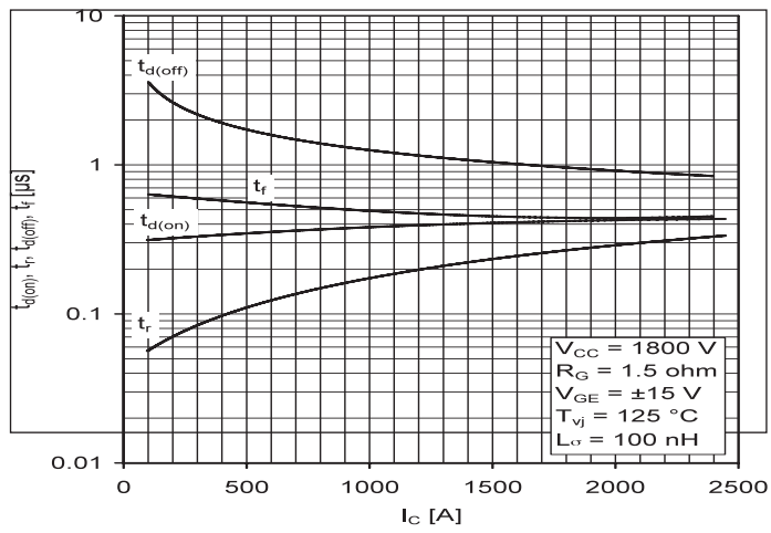
Fig. 14: Typical switching times vs. collector current
