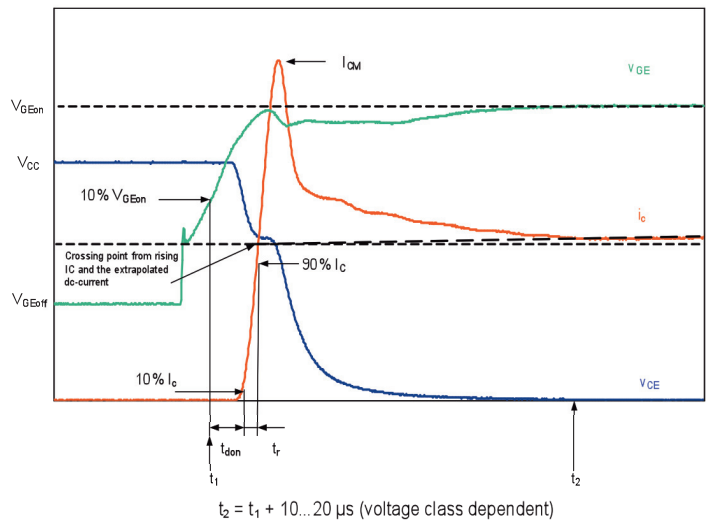
Fig. 3: Definitions of the turn-on parameters for the IGBT
