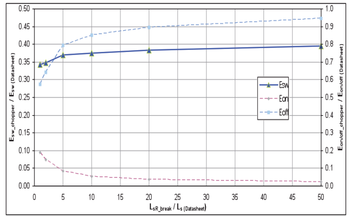
Fig. 29: Relative switching losses for resistive switching
