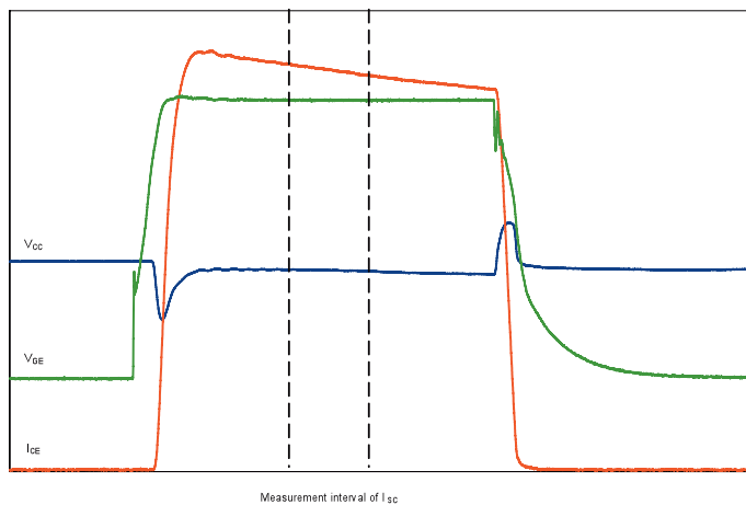
Fig. 5: Typical waveforms for Short-Circuit
