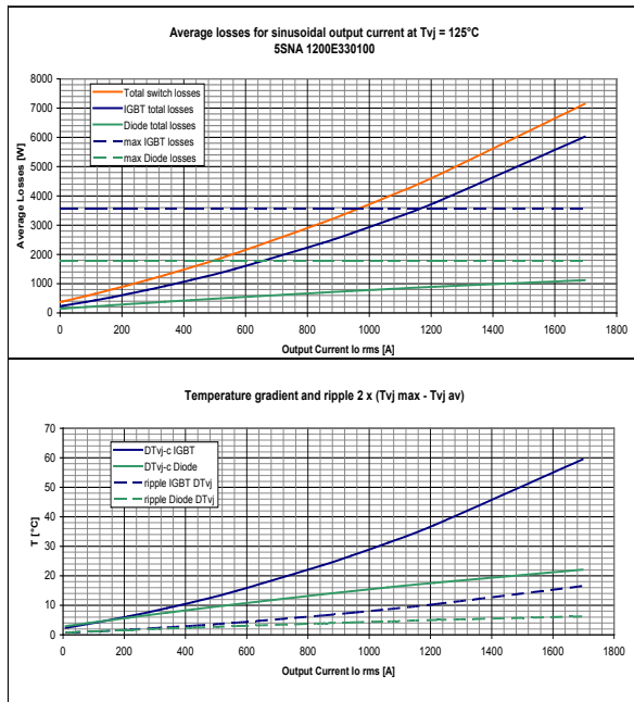
Fig. 33: Curves of losses and temperatures vs. output current
