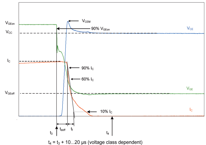
Fig. 4: Definitions of turn-off parameters for IGBTs
