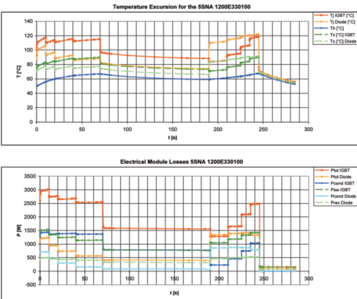
Fig. 40: Load profile calculation results in form of a temperature diagram
