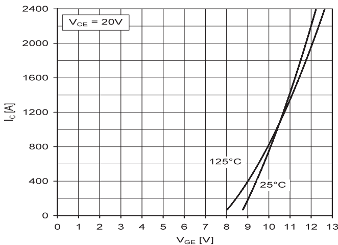
Fig. 9: Typical transfer characteristic, chip level
