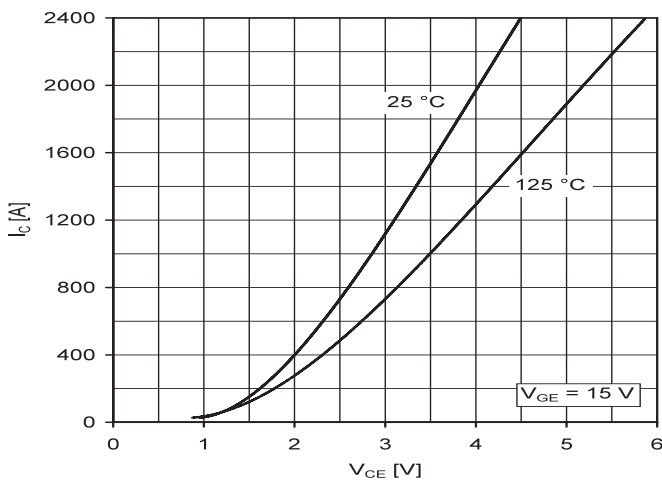
Fig. 8: Typical on-state characteristic, chip level
