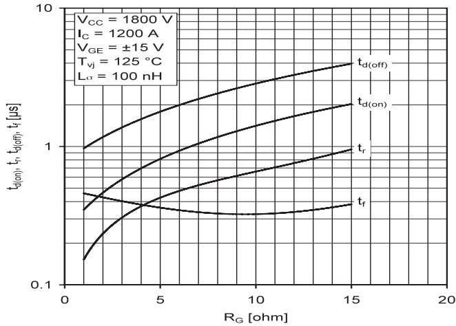
Fig. 15: Typical switching times vs. gate resistor
