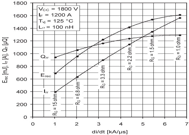
Fig. 20: Typical reverse recovery characteristics vs di/dt
