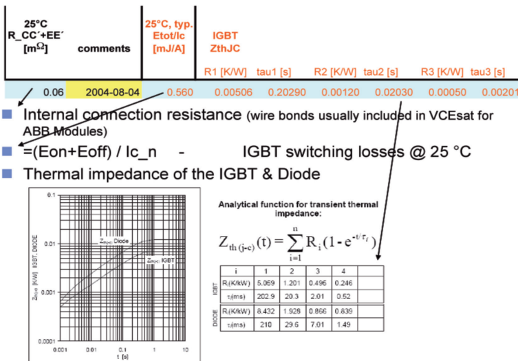
Fig. 44: Input fields for the internal resistance and the thermal impedance
