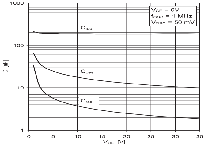
Fig. 16: Typical capacitances vs collector-emitter voltage
