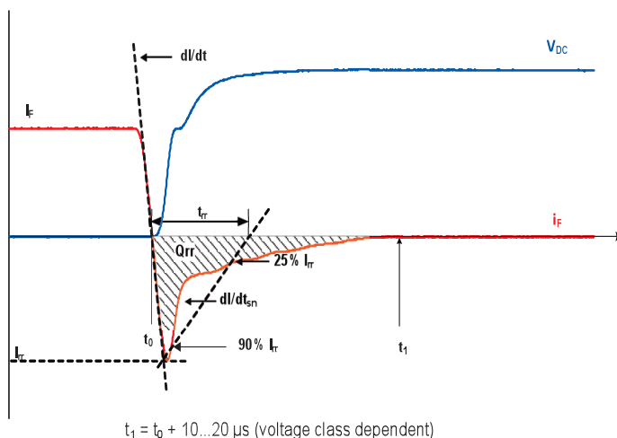
Fig. 7: Definitions for the turn-off parameters for the Diode
