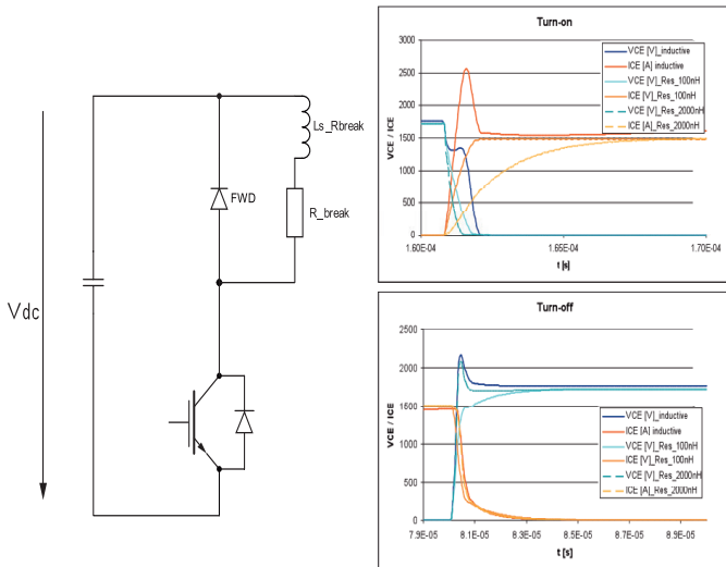
Fig. 28: Breaking Chopper schematics and switching waveforms
