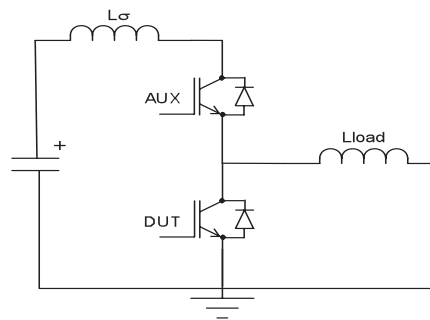
Fig. 6: Test circuit for the dynamic performance of the Diode
