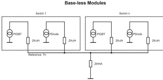
Fig. 26: Thermal equivalent block diagram for baseless devices
