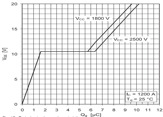
Fig. 17: Typical gate charge characteristics
