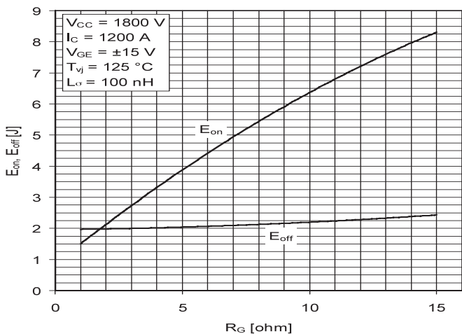
Fig. 13: Typical switching energies per pulse vs. gate resistor
