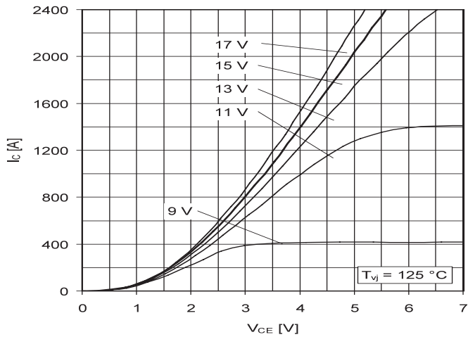
Fig. 11: Typical output characteristic, chip level
