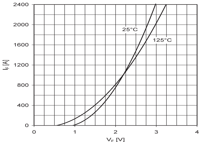
Fig. 21: Typical diode forward characteristic, chip level
