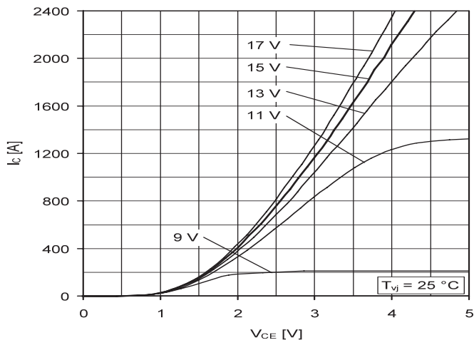
Fig. 10: Typical output characteristic, chip level
