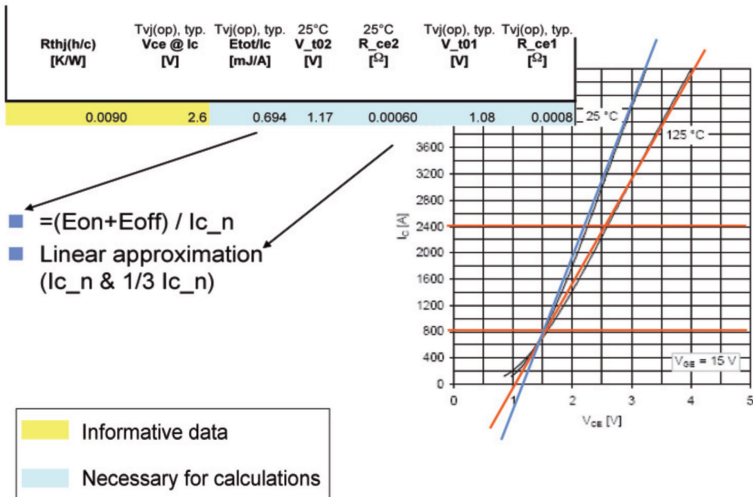
Fig. 42: Input fields for the IGBT loss characteristics
