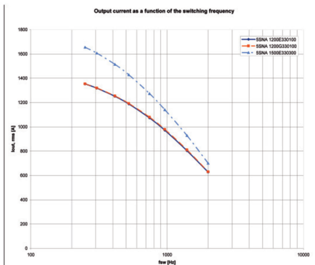
Fig. 38: Performance chart (results)
