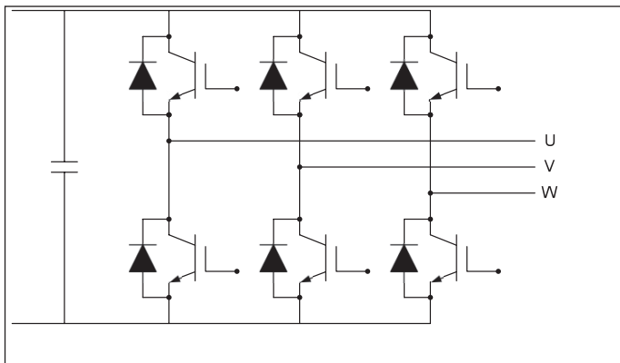
Fig 1: 2-level voltage source inverter with IGBTs
