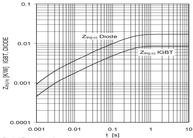
Fig. 23: Thermal impedance vs time
