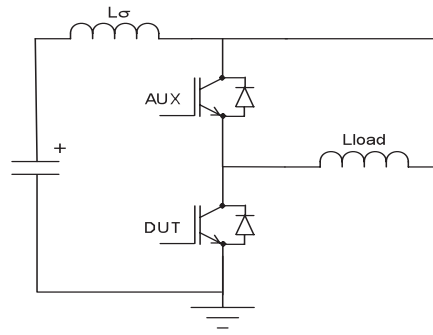
Fig. 2: Electrical circuit for testing of the dynamic performance of the IGBT
